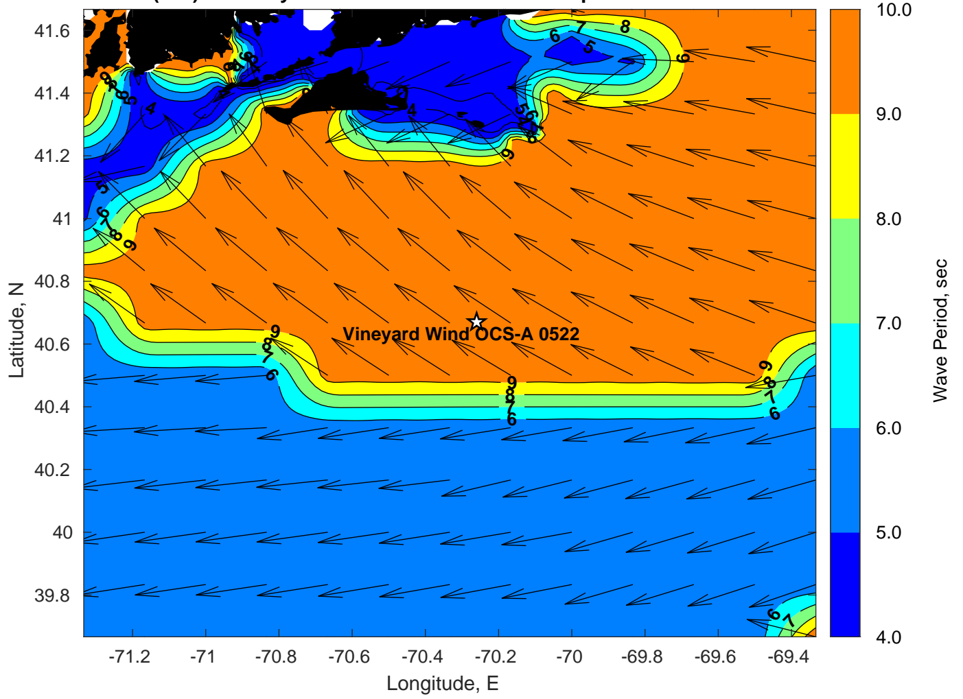
Wave Period (sec) for Vineyard Wind OCS-A 0522 at 07-Sep-2022 12:00:00
